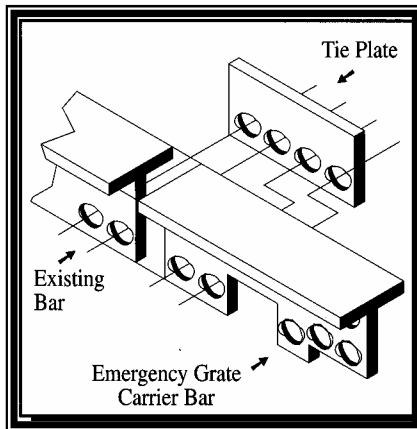
KE Emergency Grate Carrier Bar
